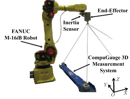
Fig. 9. FANUC M-16iB robot system.
