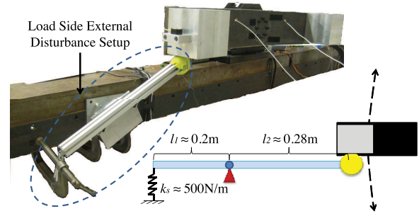
Fig. 3. Load side disturbance setup for a single-joint system.
